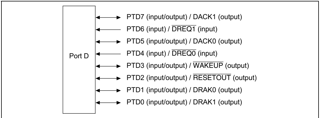
Figure 20.4 Port D
