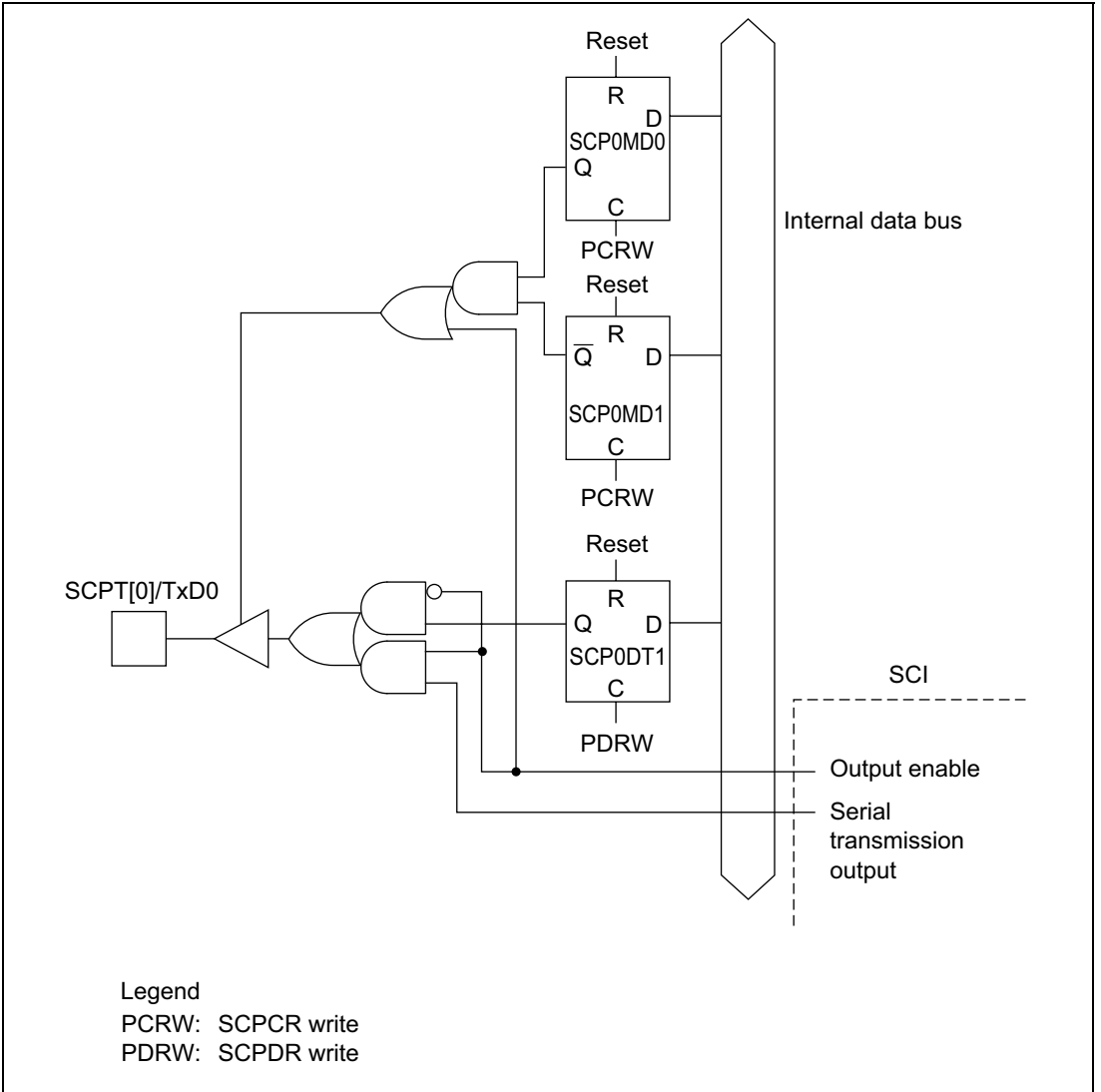
Figure 15.3 SCPT[0]/TxD0 Pin
