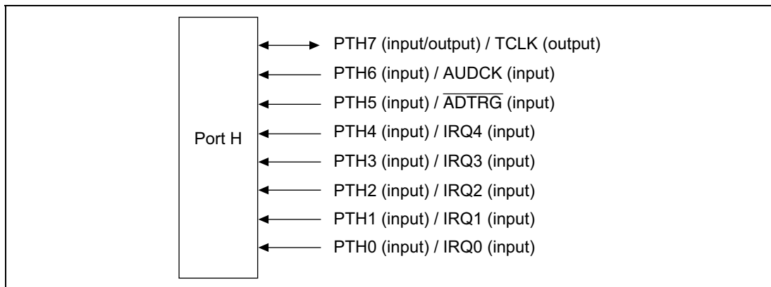
Figure 20.8 Port H
