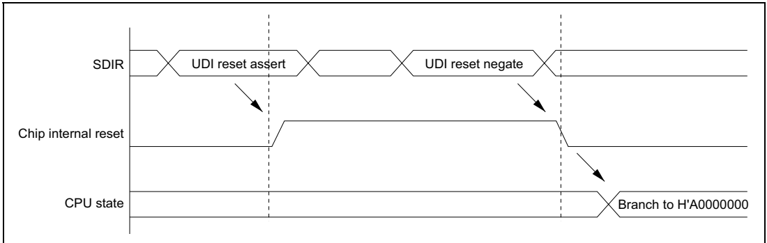
Figure 23.3 UDI Reset
