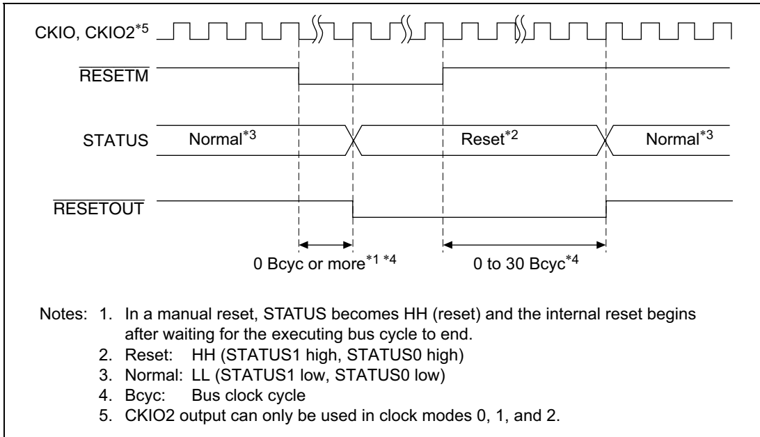
Figure 9.3 Manual Reset STATUS Output
