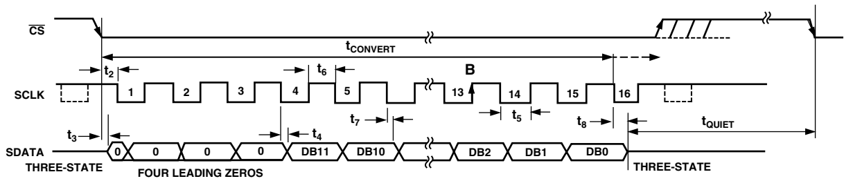
Figure 1. Serial Interface Timing Diagram
