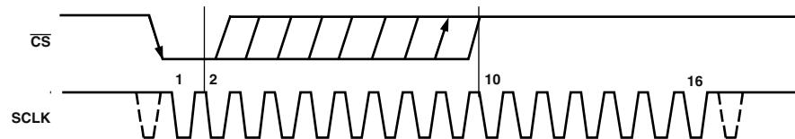
Figure 14. Entering Partial Power-Down Mode
