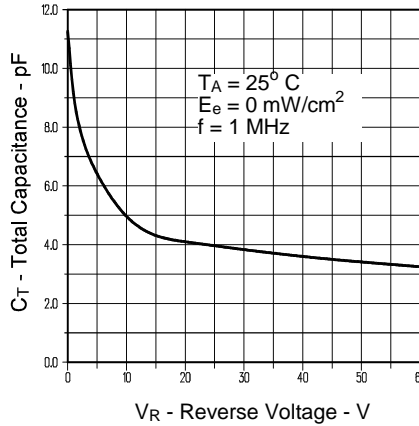
Total Capacitance vs Reverse Voltage
