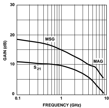
Figure 4. ATF-21186 Insertion Power Gain, Maximum Available Gain, and Maximum Stable Gain vs. Frequency. V_{DS} = 2 V, I_{DS} = 10 mA.
