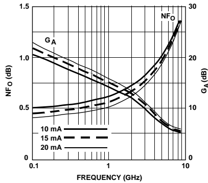
Figure 1. ATF-21186 Optimum Noise Figure and Associated Gain vs. Frequency and I_{DS} , V_{DS} = 2 V.
