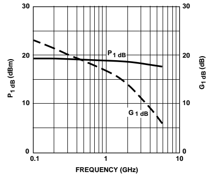
Figure 3. ATF-21186 Power Output at 1 dB Compression and 1 dB Compressed Gain vs. Frequency. V_{DS} = 3 V, I_{DS} = 70 mA.
