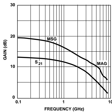
Figure 5. ATF-21186 Insertion Power Gain, Maximum Available Gain, and Maximum Stable Gain vs. Frequency. V_{DS} = 2 V, I_{DS} = 20 mA.
