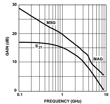
Figure 6. ATF-21186 Insertion Power Gain, Maximum Available Gain, and Maximum Stable Gain vs. Frequency. V_{DS} = 3 V, I_{DS} = 70 mA.
