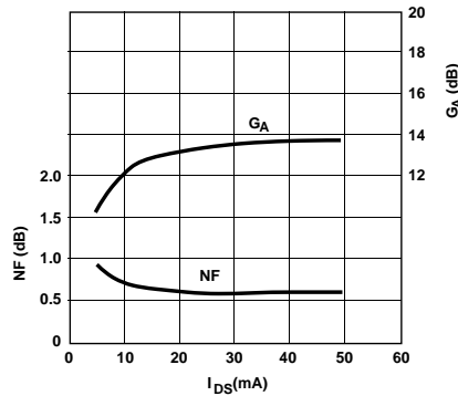
Figure 2. ATF-21186 Optimum Noise Figure and Associated Gain vs. I_{DS} , f = 2 GHz, V_{DS} = 2 V.
