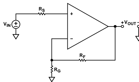
Figure 64. Noninverting Configuration
