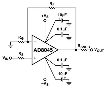
Figure 61. Noninverting Configuration
