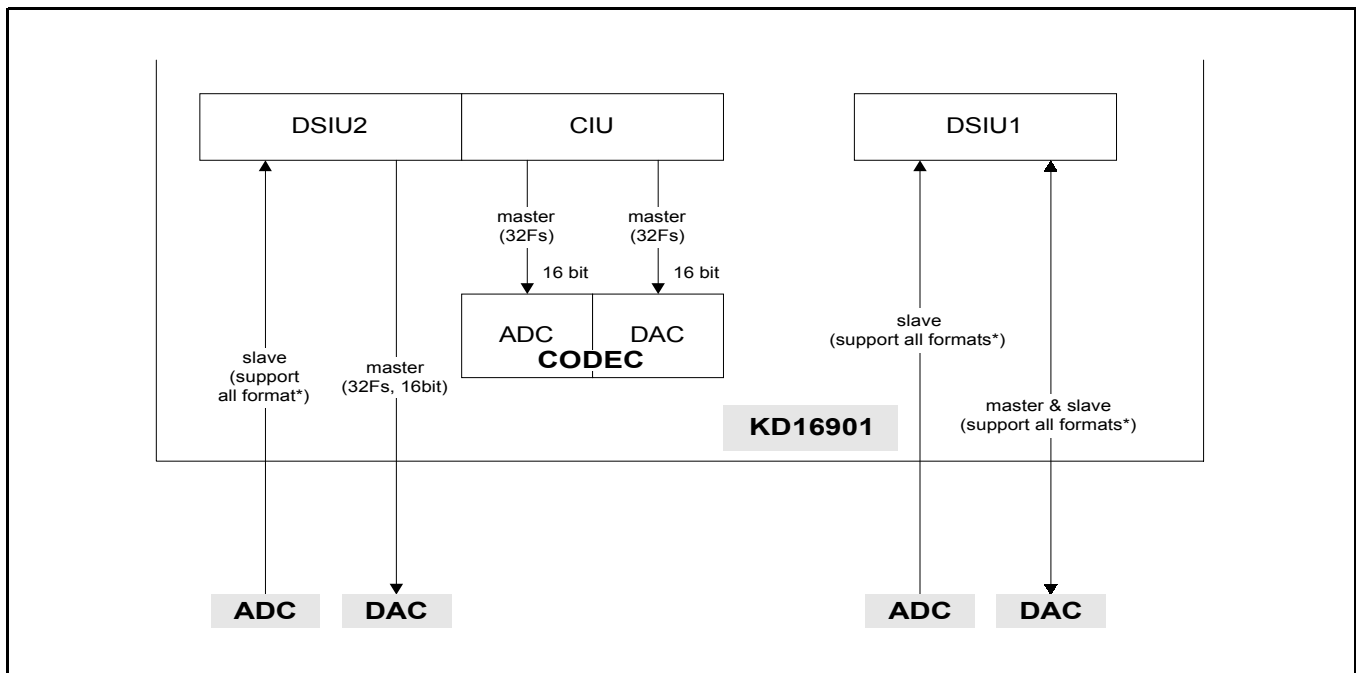
Figure 4. Digital Audio Interface Formats of the KD16901
