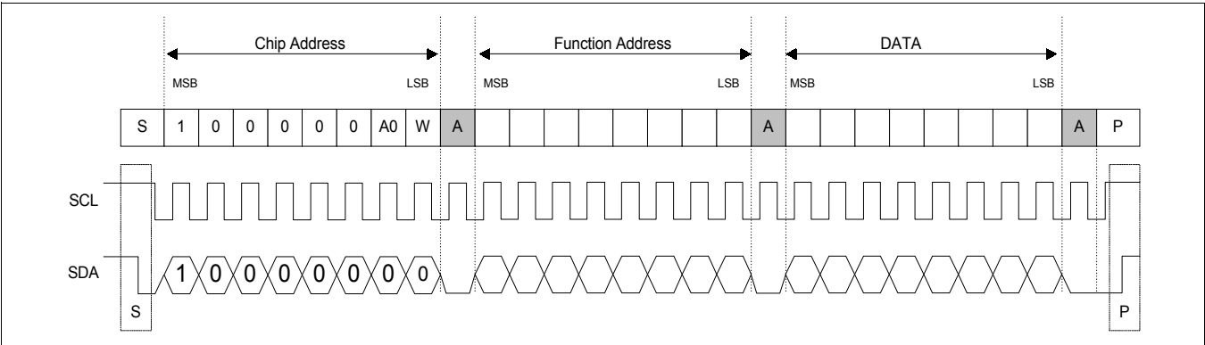
Figure 10. I²C Bus Interface Format-Write Operation (SAS = 0)
