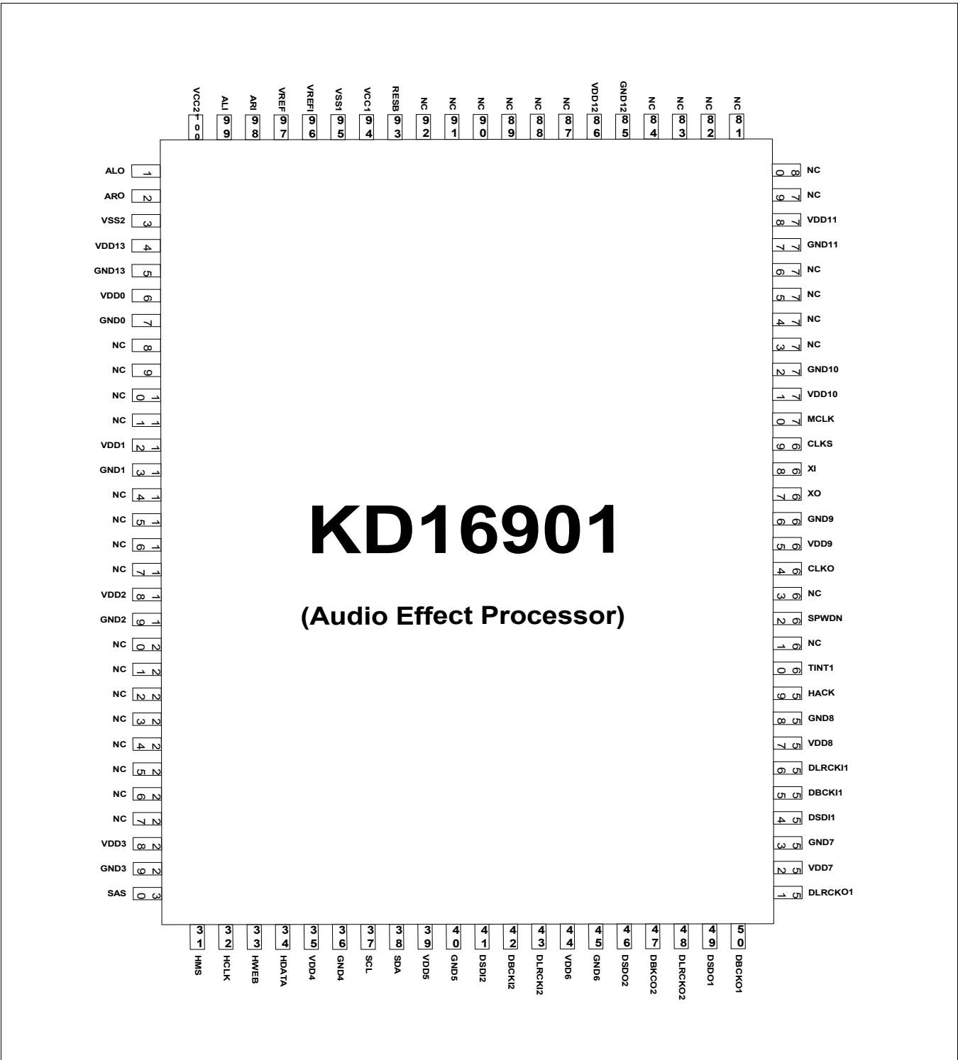
Figure 3. KD16901 Pin Assignmen
