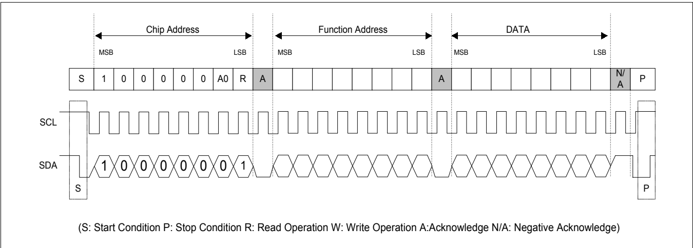
Figure 11. I²C Bus Interface Format-Read Operation (SAS = 0)
