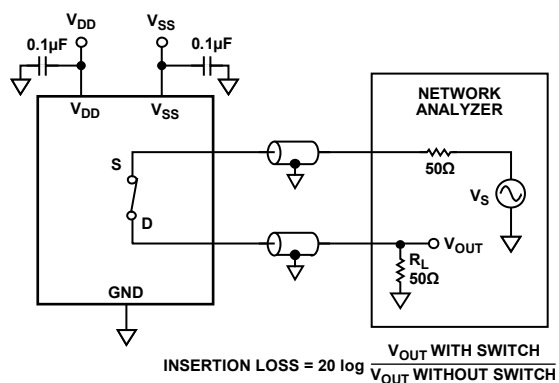
Figure 22. Bandwidth
