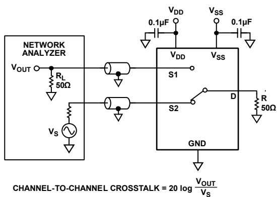
Figure 21. Channel-to-Channel Crosstalk
