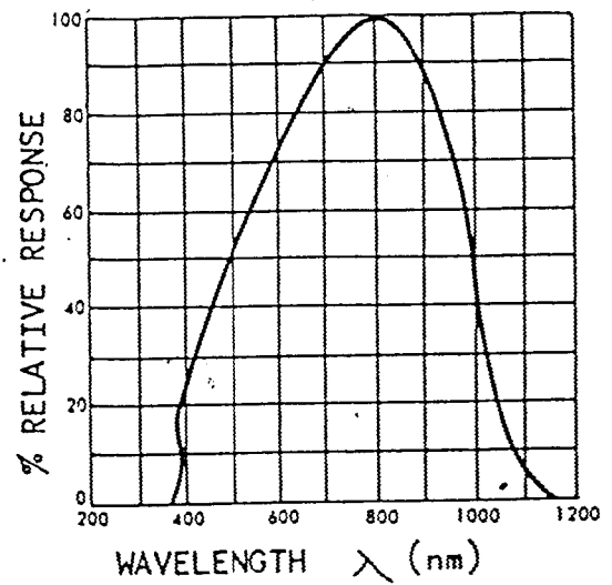
SPECTRAL CHARACTERISTICS
