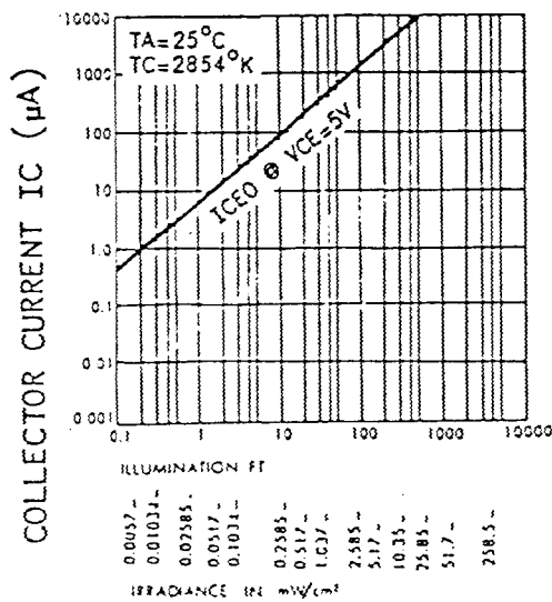
PHOTO CURRENT CHARACTERISTICS
