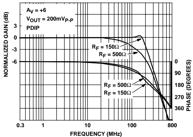
FIGURE 27. FREQUENCY RESPONSE
