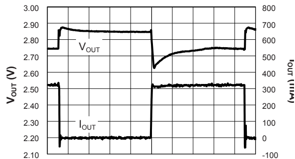
Load Transient Response 300mA
