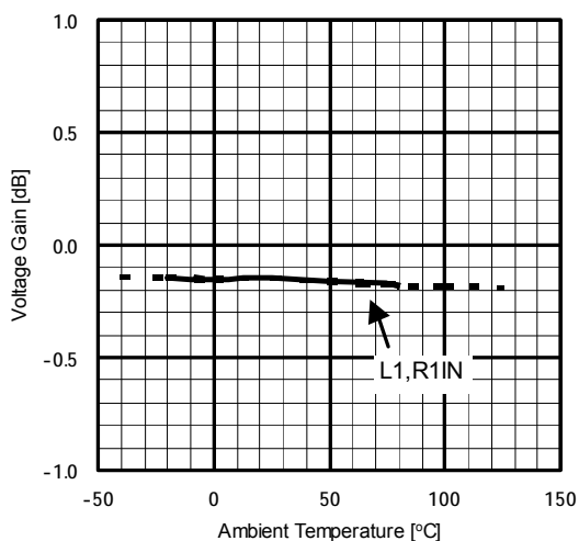
Voltage Gain vs. Ambient Temperature V^+=12V, V_{in}=1V, f=1kHz, Vol=0dB
