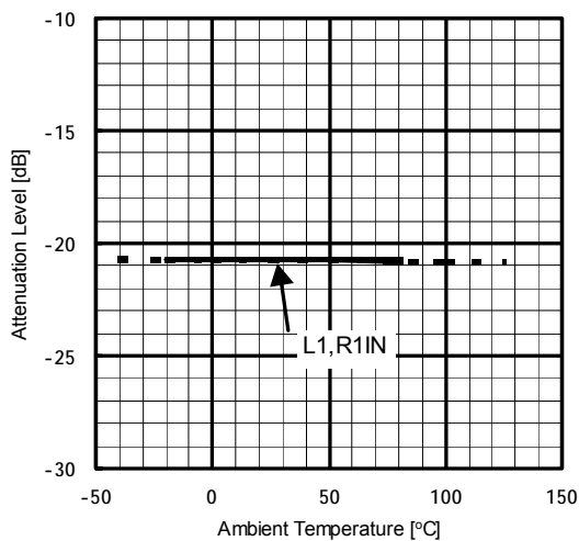
Attenuation Level vs. Ambient Temperature V^+=12V, V_{in}=1V, f=1kHz, Vol=-20dB
