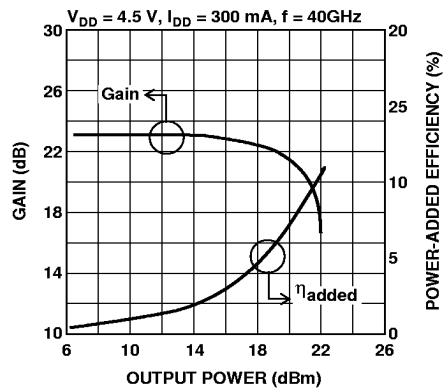
Figure 10. Gain Compression and Efficiency Characteristics. [2]
