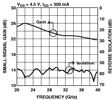
Figure 2. Typical Gain and Isolation vs. Frequency.[1]
