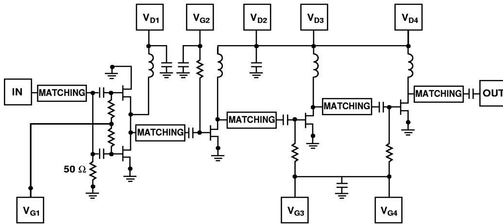
Figure 1. HMMC-5040 Simplified Schematic Diagram.
