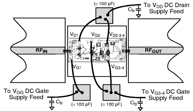
Figure 12b. Separate first-stage gate bias supply for any multiplier or amplifier application. This diagram shows an optional variation to the V_{G2} jumper-wire bonding scheme presented in (a).
