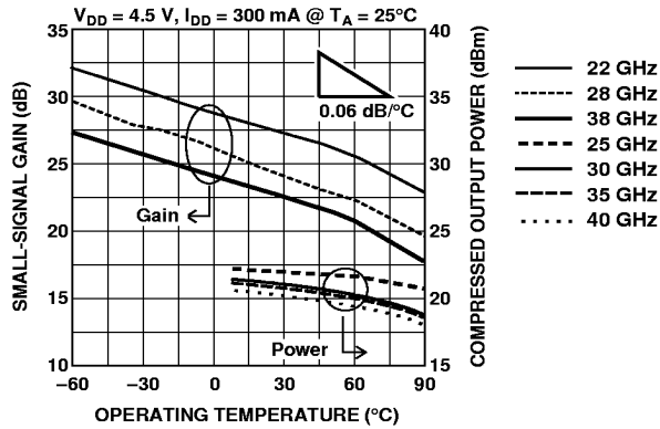
Figure 6. Small-Signal Gain [3] and Compressed Power [1] vs. Temperature.
