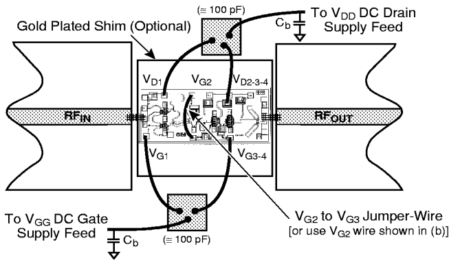
Figure 12a. Single drain and single gate supply assembly for tripler and standard amplifier applications.
