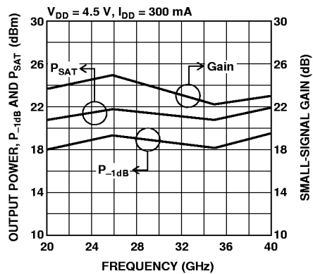
Figure 11. Output Power and Gain vs. Frequency Characteristics. [2]
