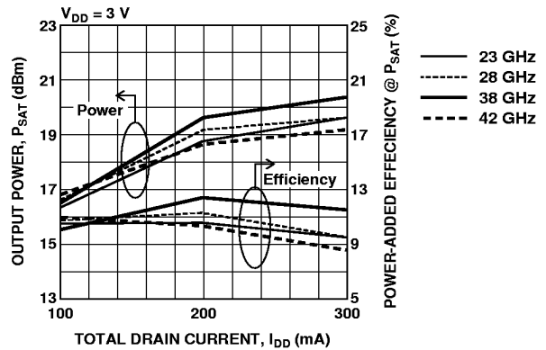
Figure 9. Output Power [1] and Efficiency vs. Drain Current with V_{DD} = 3 V.
