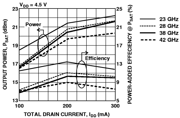
Figure 8. Output Power [1] and Efficiency vs. Drain Current with V_{DD} = 4.5 V.
