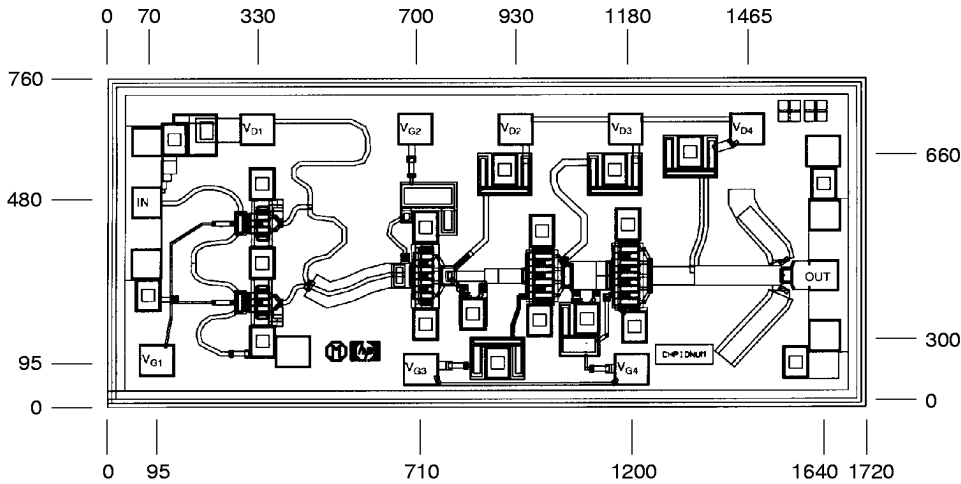
Figure 13. HMMC-5040 Bonding Pad Locations. (Dimensions in micrometers)
