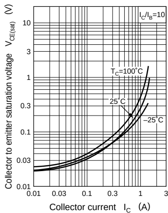
V_{CE(\text{sat})} - I_C
