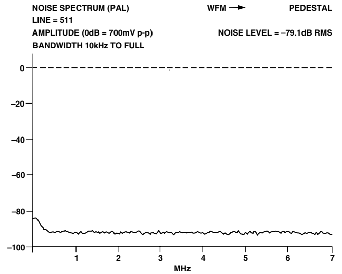
Figure 145. PAL Noise Spectrum: Pedestal
