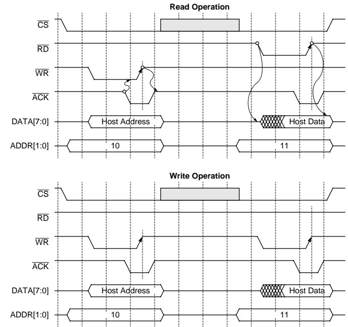
Figure 18. Asynchronous Operation of the Host Interface
