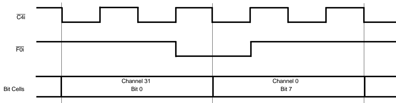
Figure 5. Frame Alignment
