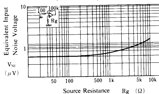
Equivalent Input Noise Voltage vs. Source Resistance
