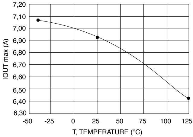
Figure 14. Current Limitation
