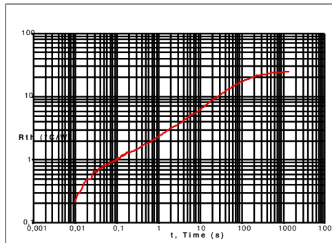
Figure 23 shows the thermal response with the device soldered on to the test PCB described on figure 22.
