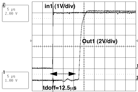
Figure 18. Output ON Delay
