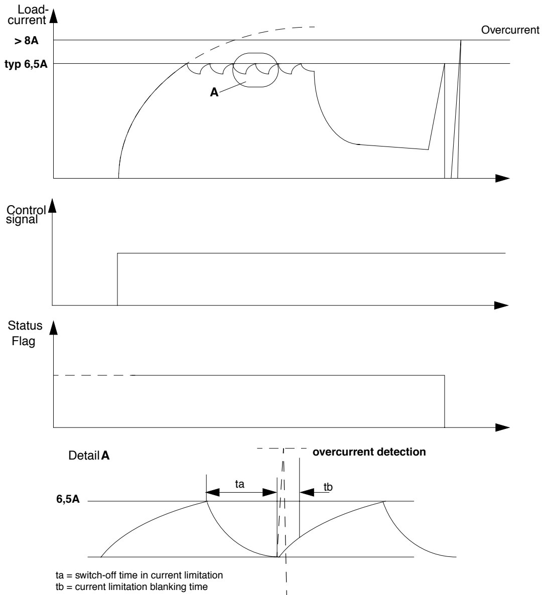
Figure 5. Current Limitation
