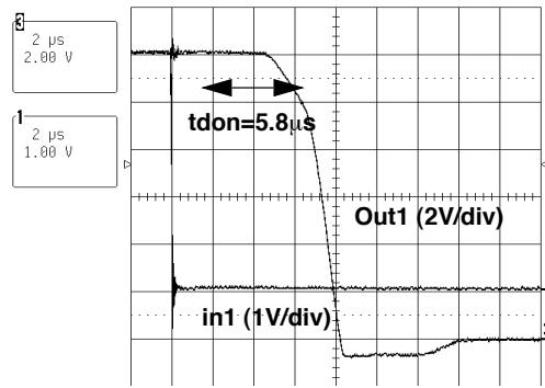
Figure 19. Output OFF Delay
