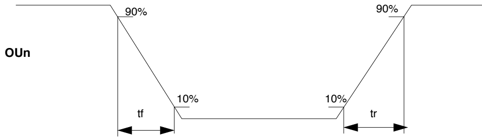
Figure 4. Output Switching Time
