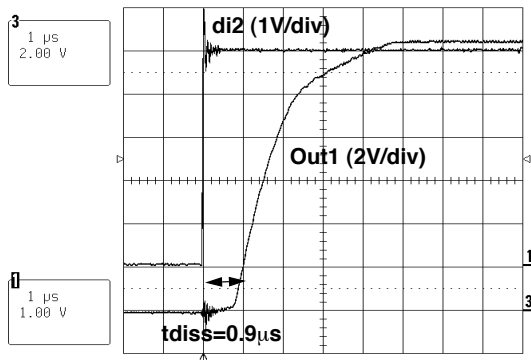
Figure 20. Disable Delay Time
