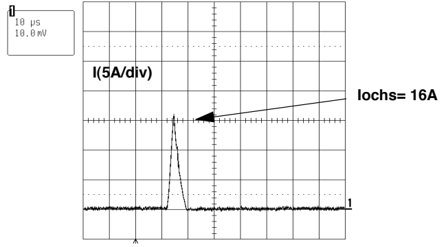
Figure 21. High side Overcurrent Detection
