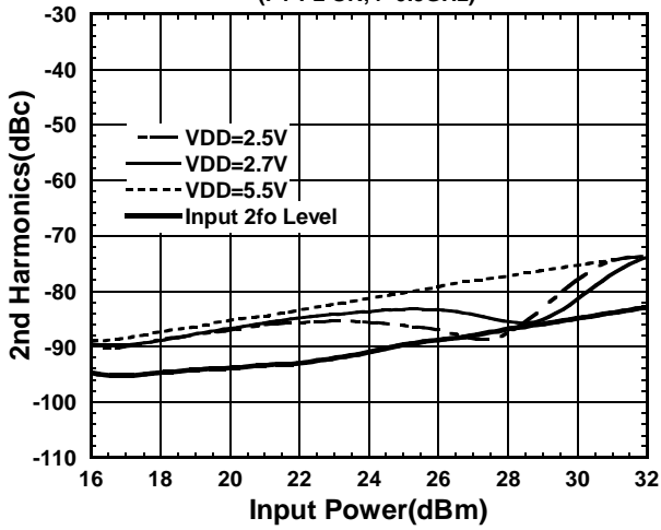
2nd Harmonics vs. Input Power (P1-P2 ON, f=0.9GHz)
