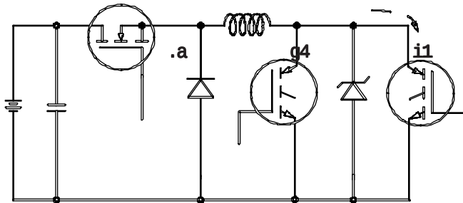
Fig. 13a - Load Test Circuit
