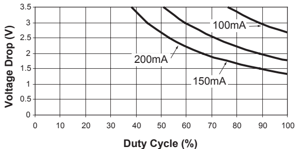
Device Duty Cycle vs. V_{DROP} V_{OUT} = 2.5V @ 85 \text{ degrees C}
