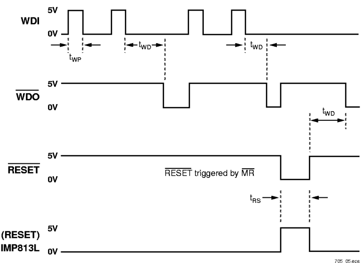
Figure 2. Watchdog Timing
