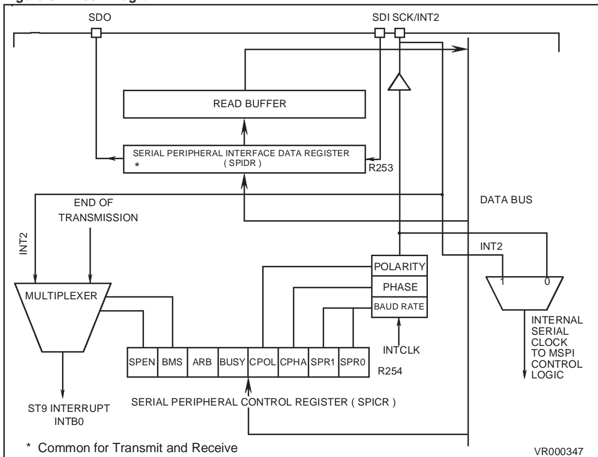
Figure 62. Block Diagram
