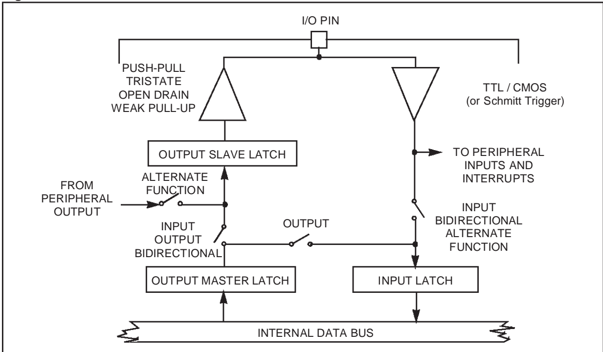
Figure 49. Input Configuration
