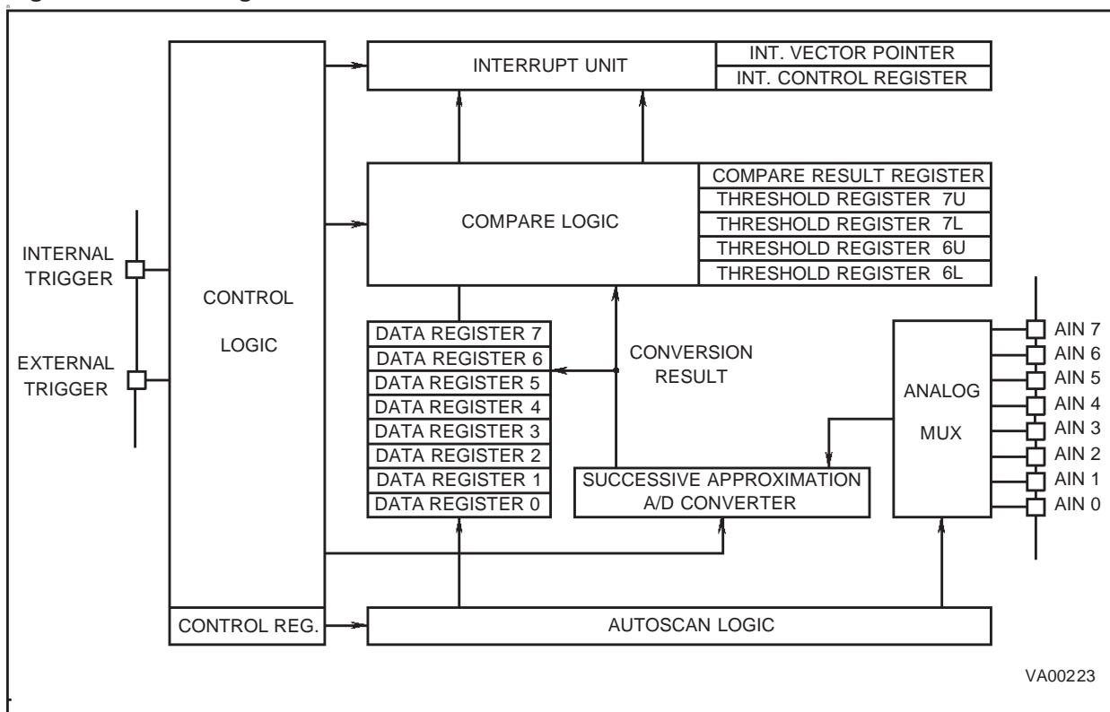
Figure 83. Block Diagram
