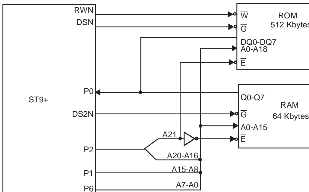
Figure 45. Application Example
