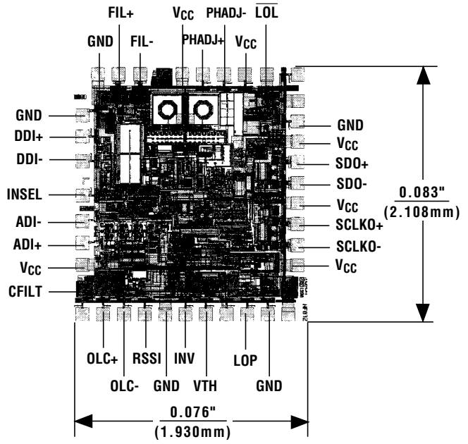
Chip Topography
