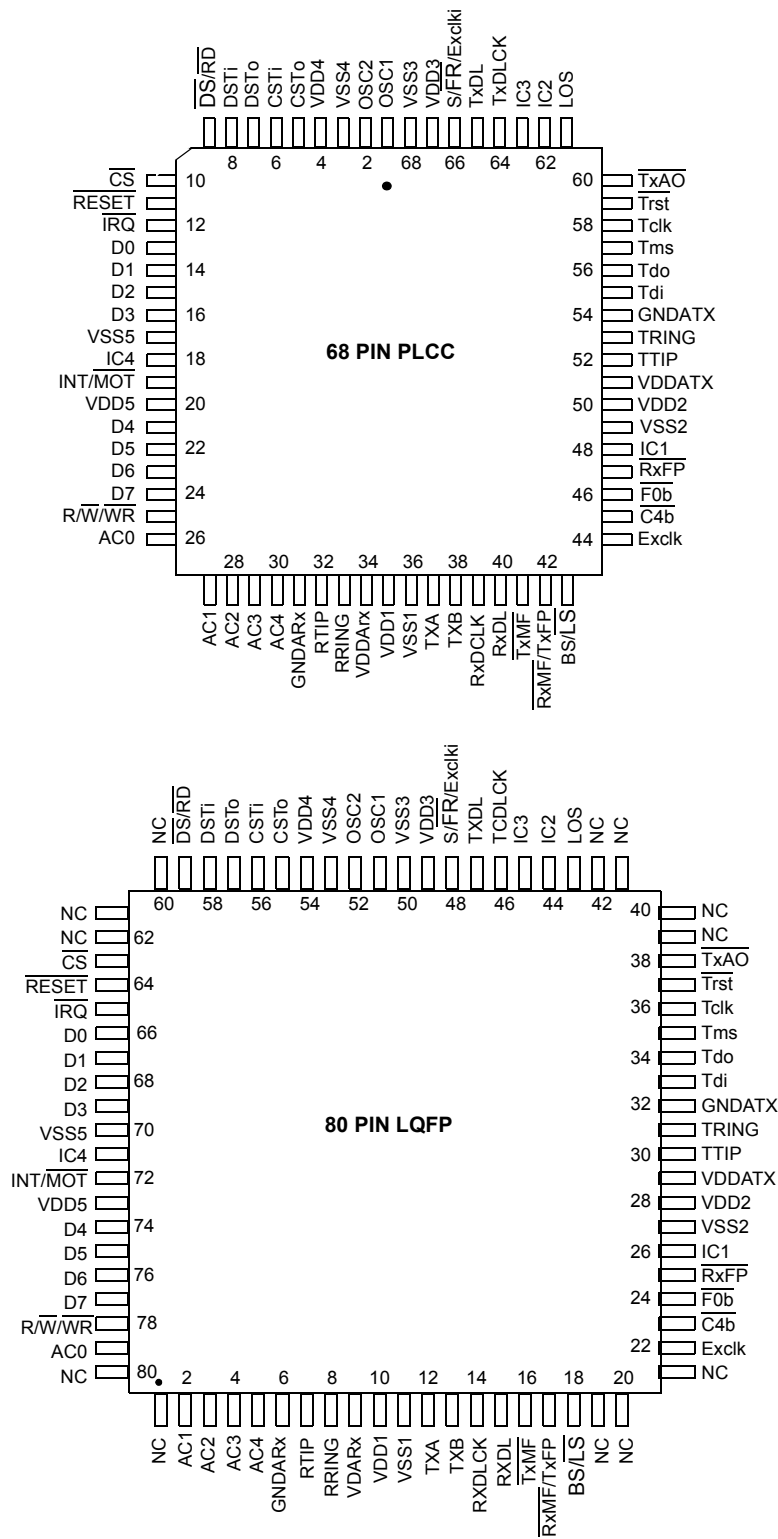
Figure 2 - Pin Connections
