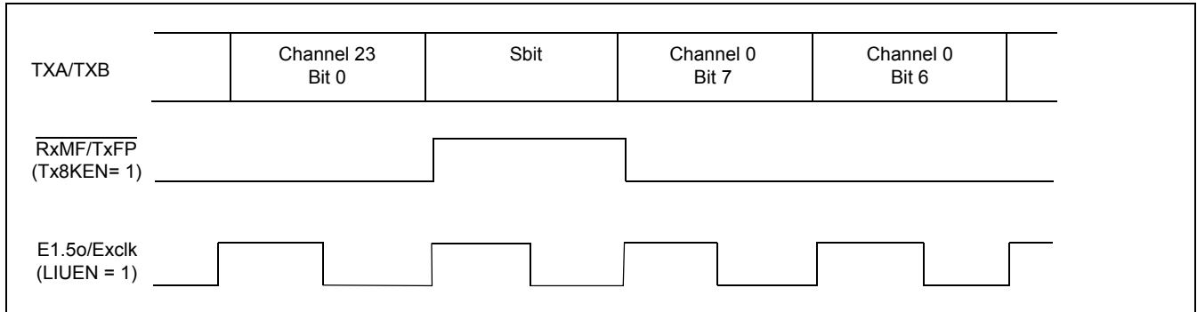
Figure 33 - TXA/TXB Functional Timing (T1 mode)
