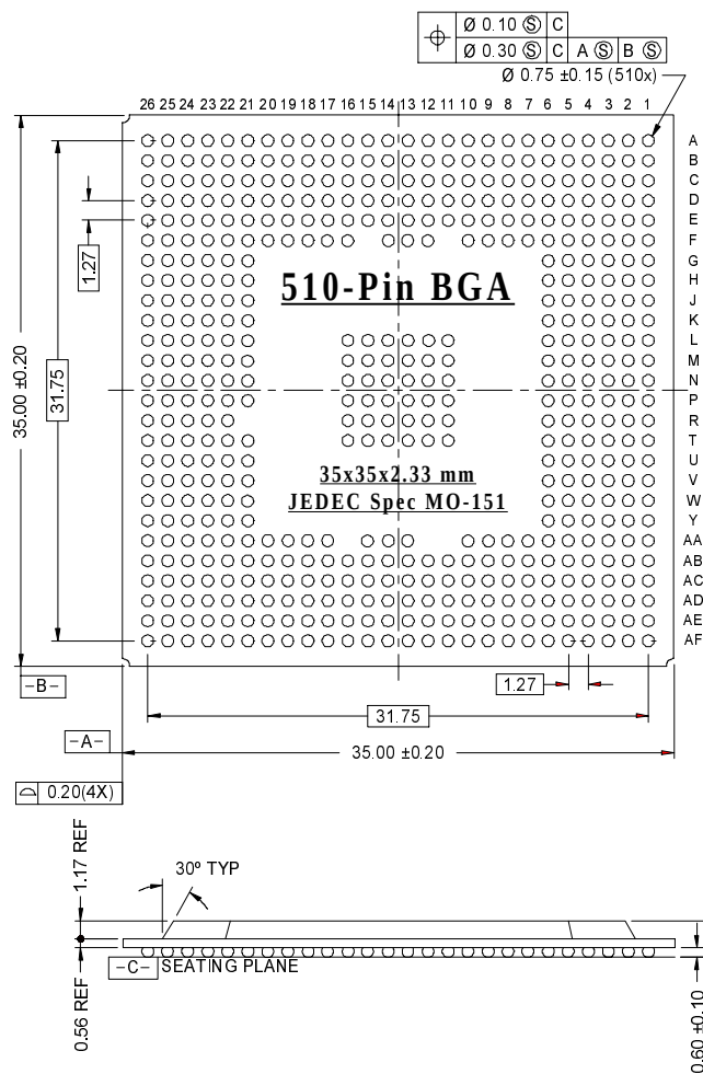
Figure 9. Mechanical Specifications - 510-Pin Ball Grid Array Package
