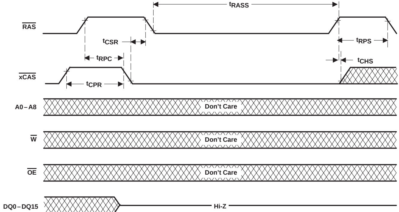
Figure 12. Self-Refresh-Cycle Timing
