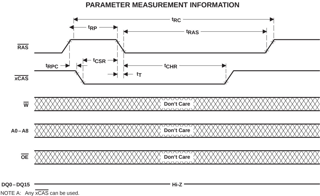
Figure 11. Automatic-CBR- Refresh-Cycle Timing
