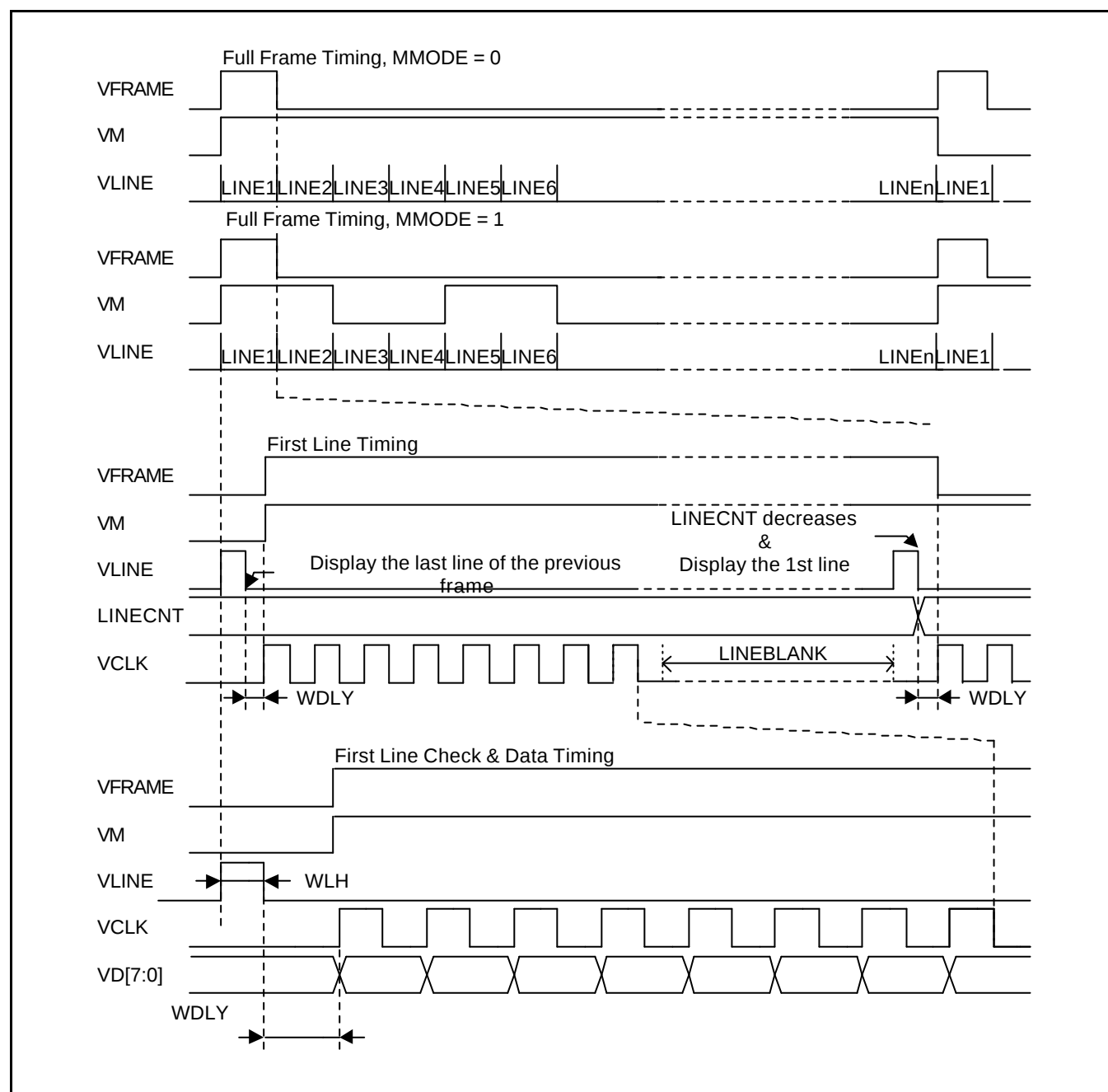
Figure 12-3. 8-bit Single Scan Display Type LCD Timing
