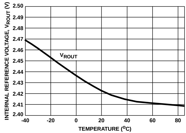
FIGURE 10. INTERNAL REFERENCE VOLTAGE ( V_{ROUT} ) vs TEMPERATURE
