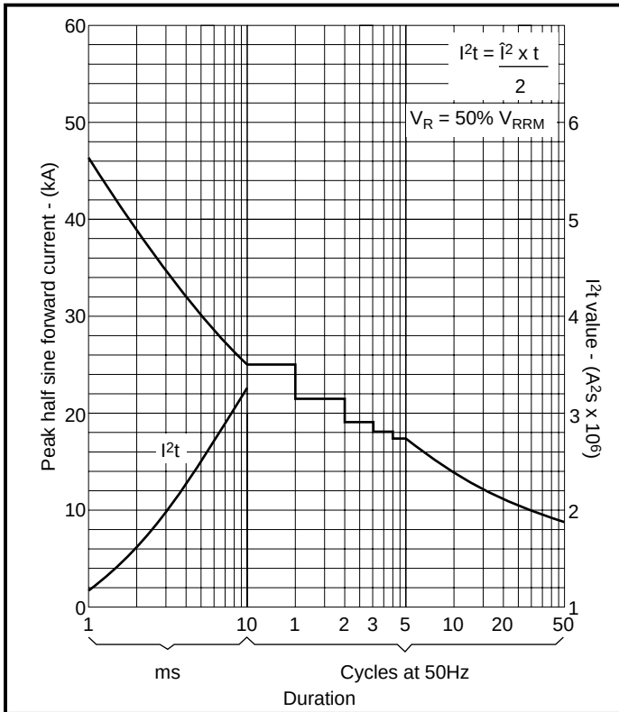
Fig.4 Surge (non-repetitive) forward current vs time (with 50% V_{RRM} at T_{case} 175^{\circ}C )
