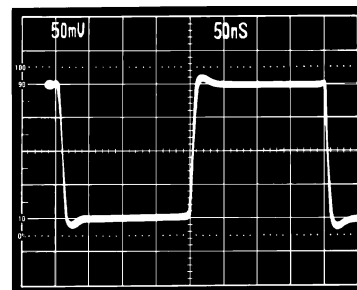
Figure 22c. Inverter Small Signal Pulse Response
