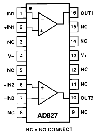
16-Pin Small Outline (R) Package
