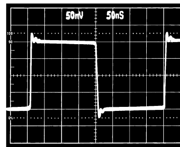
Figure 21c. Follower Small Signal Pulse Response
