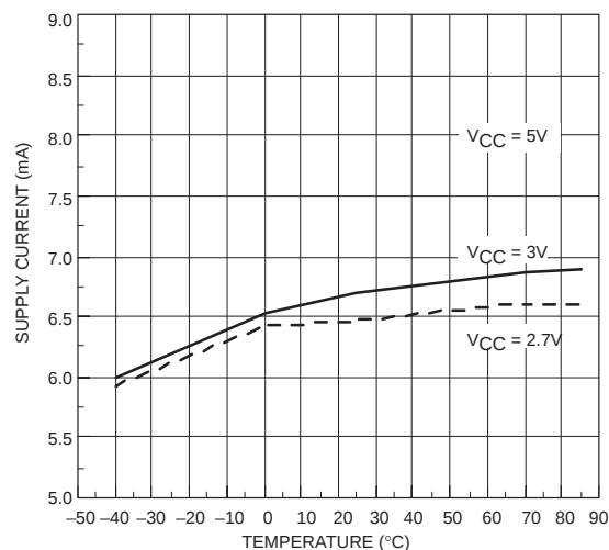
Supply Current vs Temp and Supply Voltage
