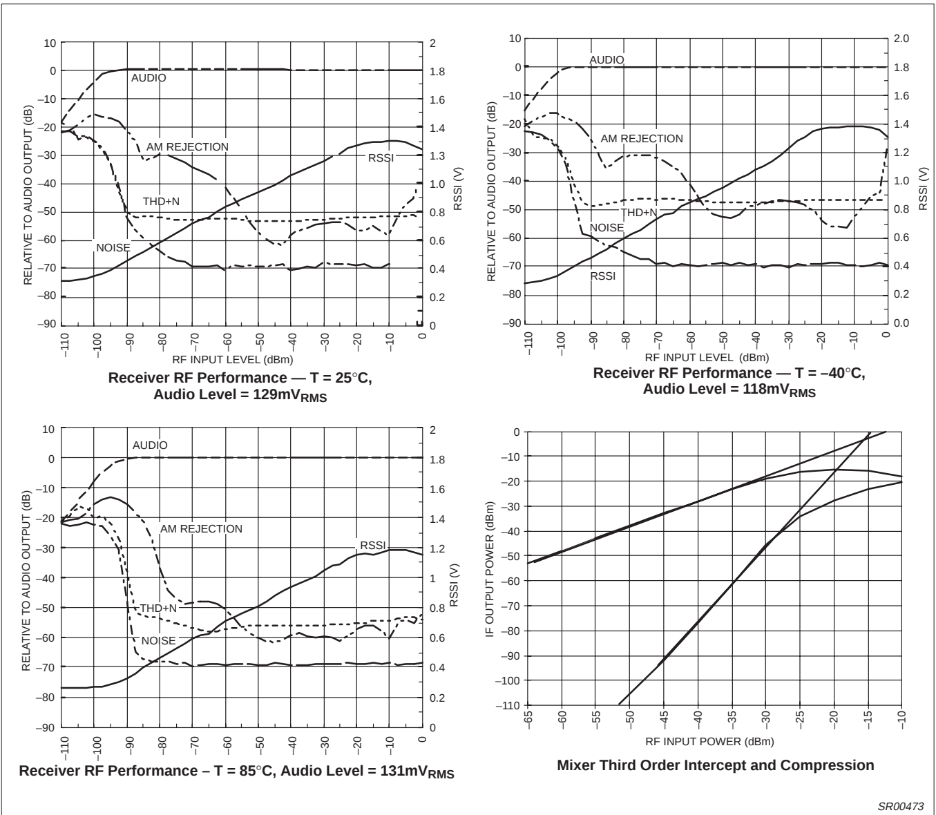
Figure 4. Performance Characteristics
