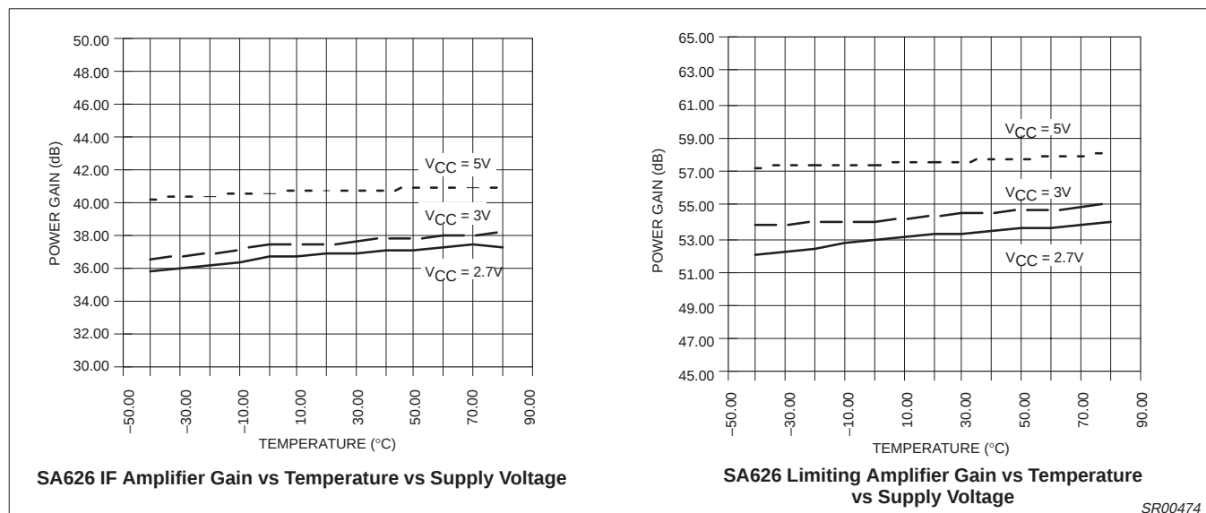
Figure 5. Performance Characteristics
