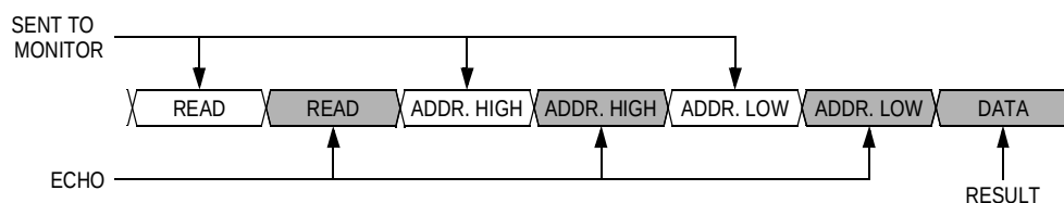
Figure 10-4. Read Transaction
