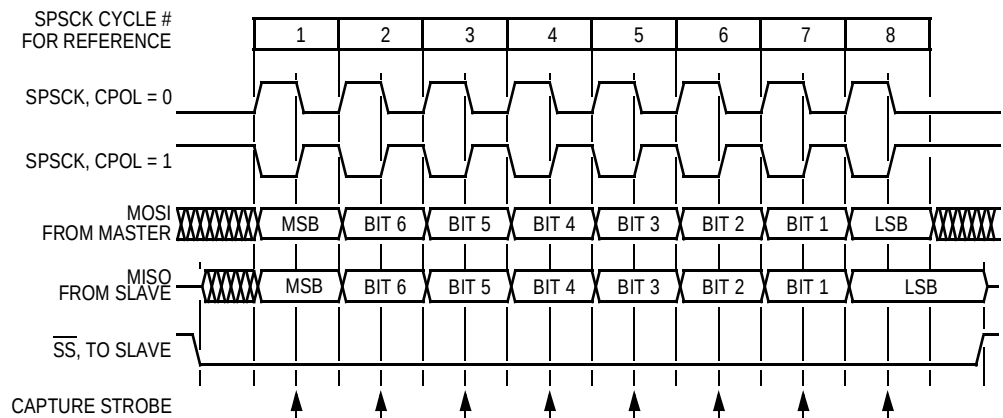
Figure 13-6. Transmission Format ( \overline{\text{CPHA}} = 1 )
