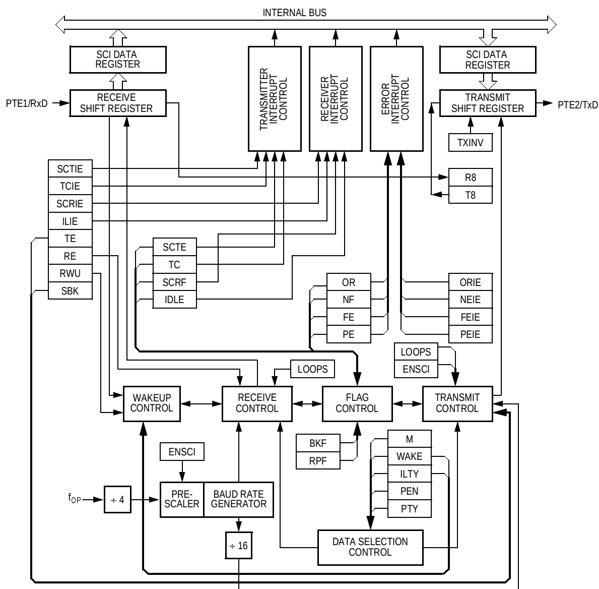
Figure 14-1. SCI Module Block Diagram
