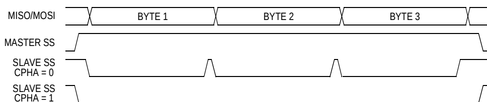
Figure 13-5. \overline{CPHA}/\overline{SS} Timing
