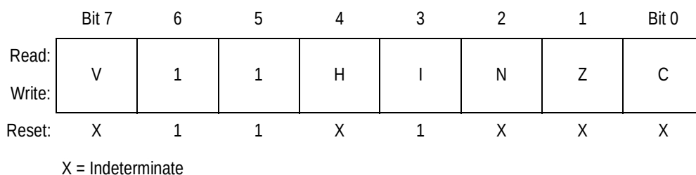
Figure 6-6. Condition Code Register (CCR)
