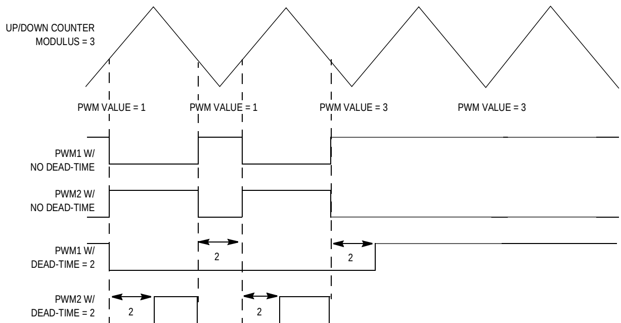
Figure 9-15. Dead-Time at Duty Cycle Boundaries
