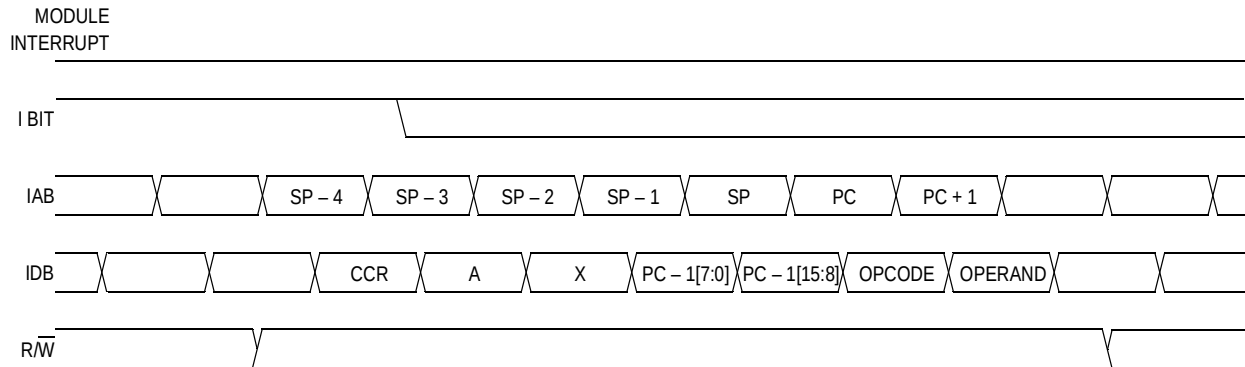
Figure 7-9. Interrupt Recovery
