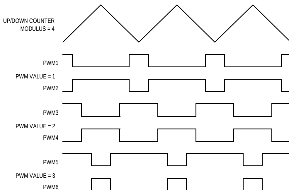
Figure 9-17. Ideal Complementary Operation (Dead-Time = 0)
