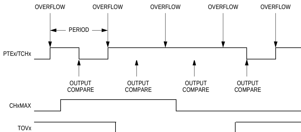
Figure 12-8. CHxMAX Latency
