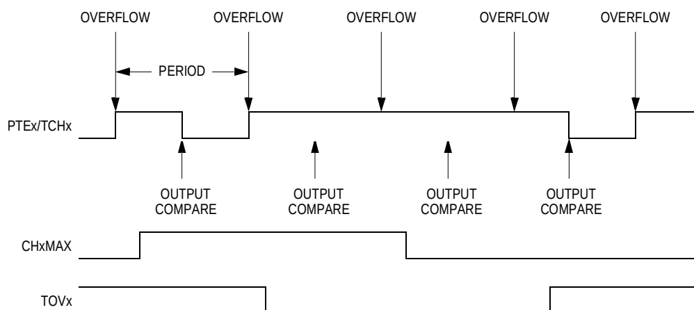
Figure 11-8. CH x MAX Latency
