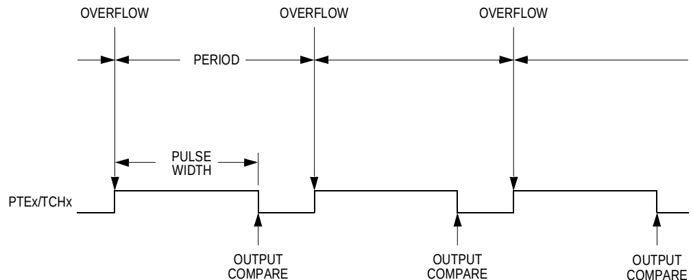
Figure 11-3. PWM Period and Pulse Width
