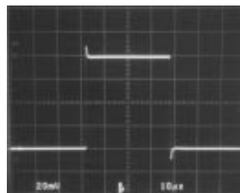
Small-Signal Response
