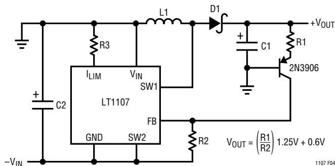
Figure 4. Negative-to-Positive Converter
