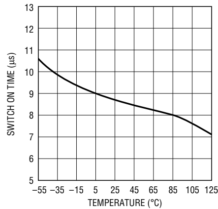
Switch ON Time Step-Down Mode
