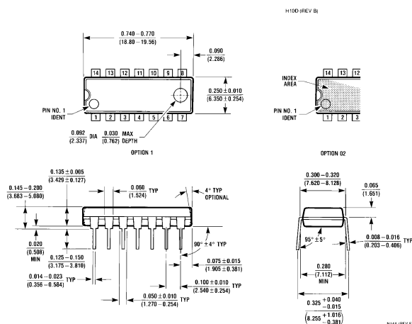
Molded Dual-In-Line Package (N) Order Number LM733CN NS Package Number N14A
