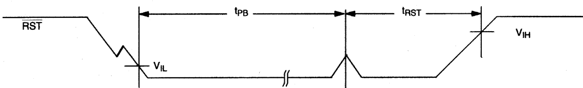
TIMING DIAGRAM: POWER-UP Figure 4
