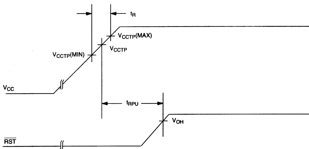
TIMING DIAGRAM: POWER-UP Figure 4
