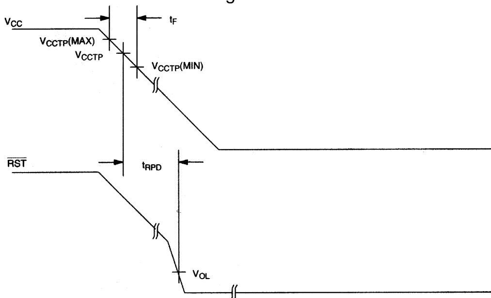
TIMING DIAGRAM: POWER-DOWN Figure 5
