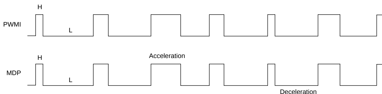
Timing Chart 1-15
