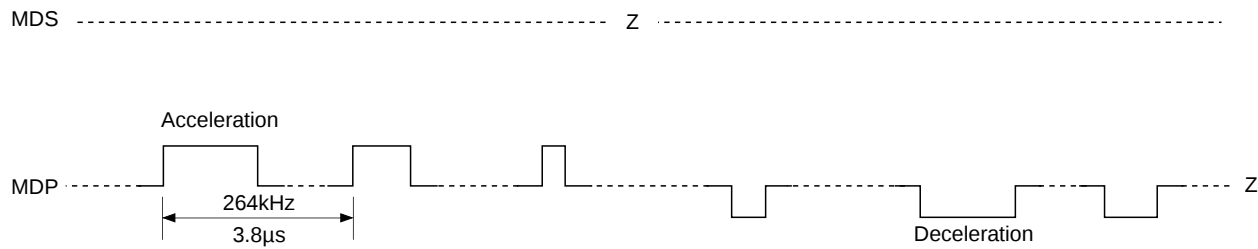
Timing Chart 1-11
