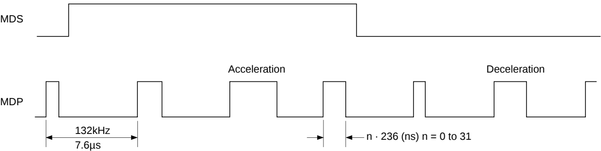
Timing Chart 1-10
