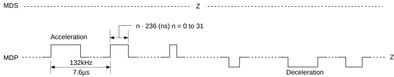
Timing Chart 1-9
