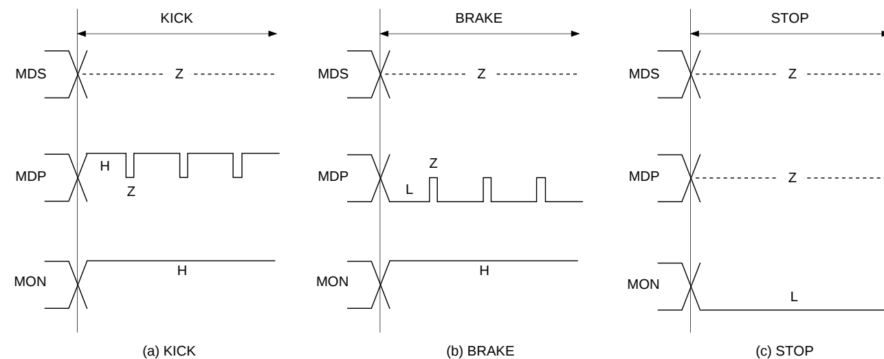
Timing Chart 1-4
