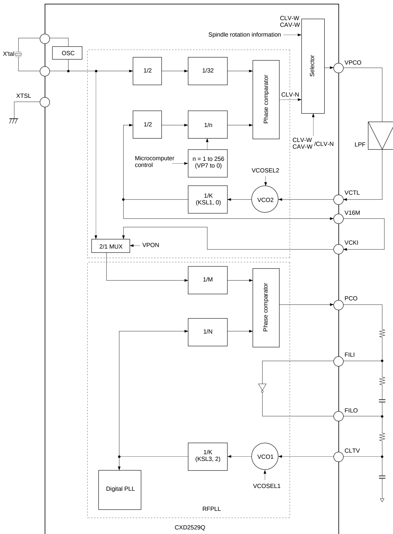
Block Diagram 4-1
