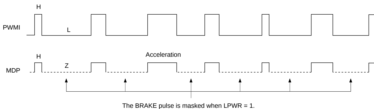
Timing Chart 1-15
