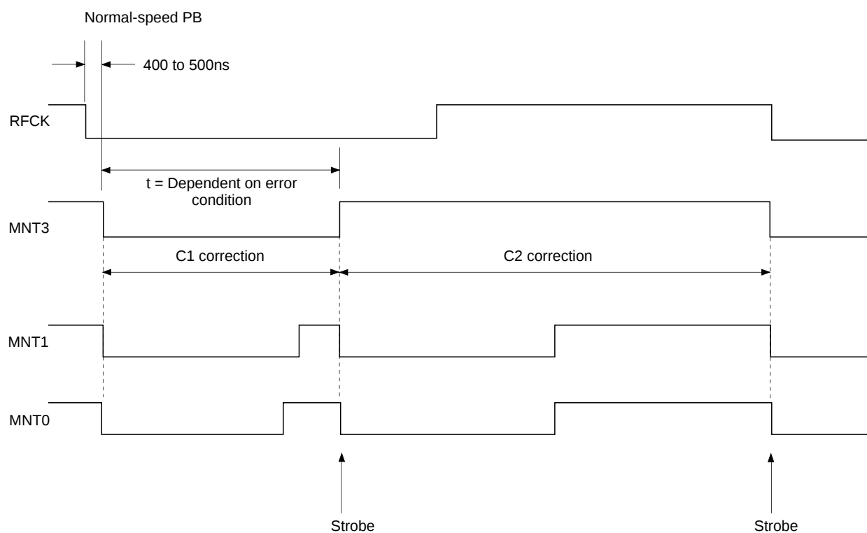
Timing Chart 4-1
