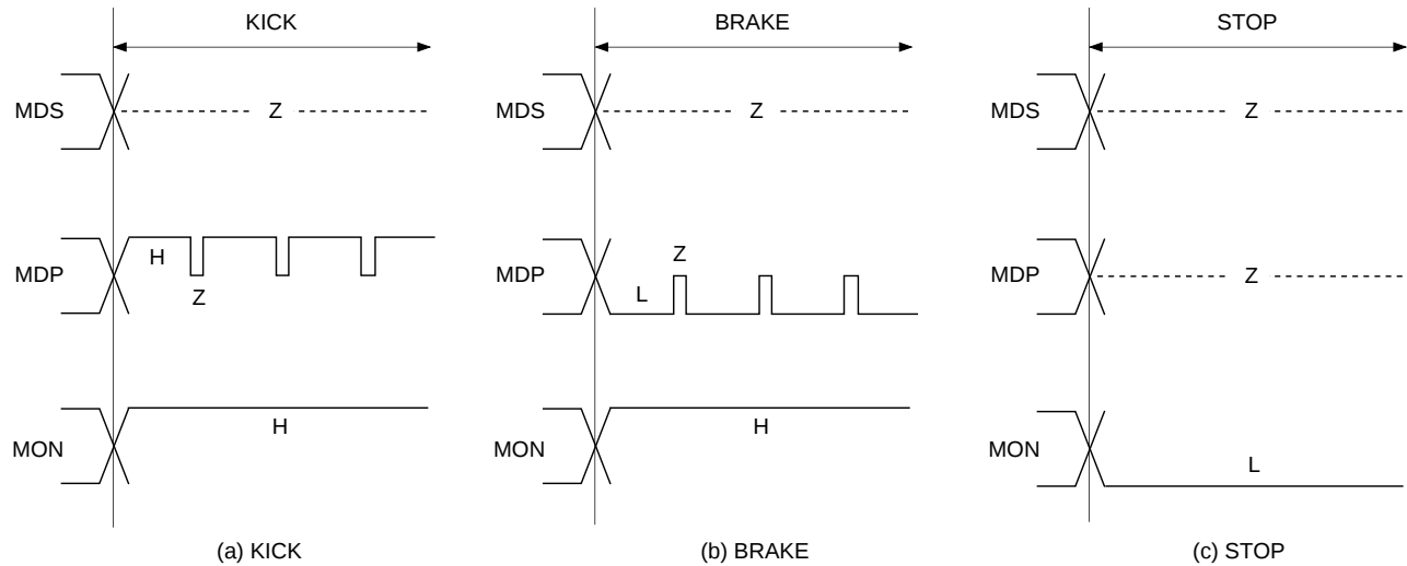
Timing Chart 1-3
