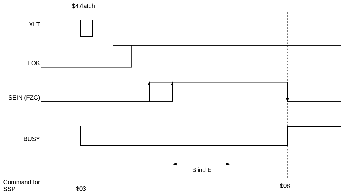
Fig. 4-3-(b). Auto Focus Timing Chart
