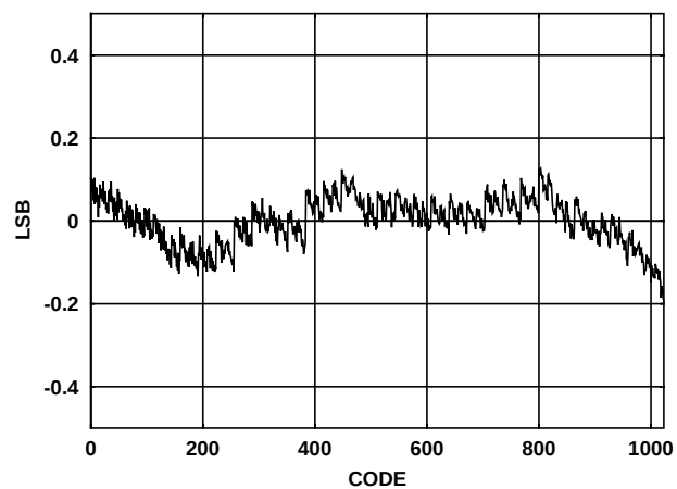
FIGURE 37. INTEGRAL NONLINEARITY
