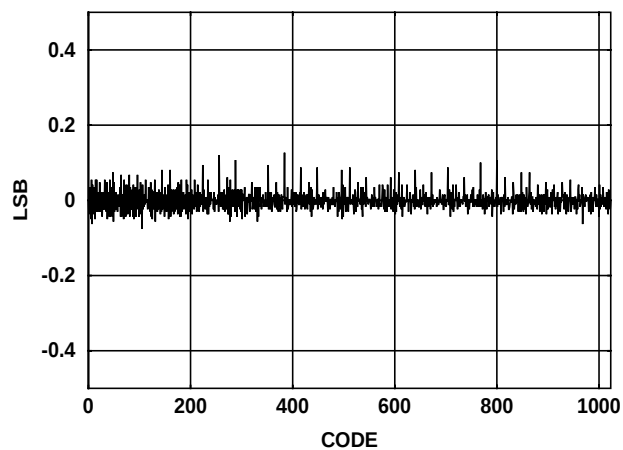
FIGURE 36. DIFFERENTIAL NONLINEARITY
