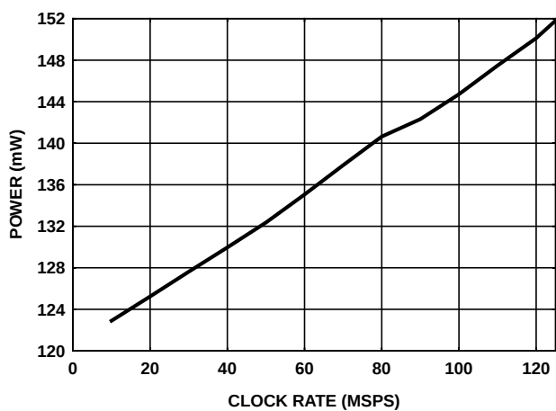
FIGURE 38. POWER vs CLOCK RATE, f_{\text{CLK}}/f_{\text{OUT}} = 10 , I_{\text{OUT}} = 20\text{mA}
