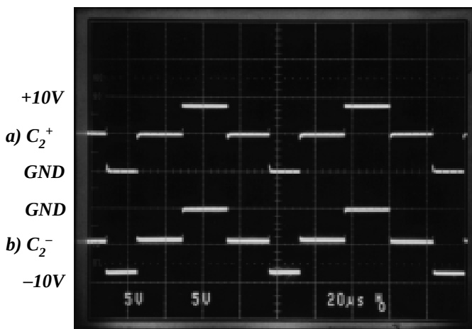
Figure 11. Charge Pump Waveforms
