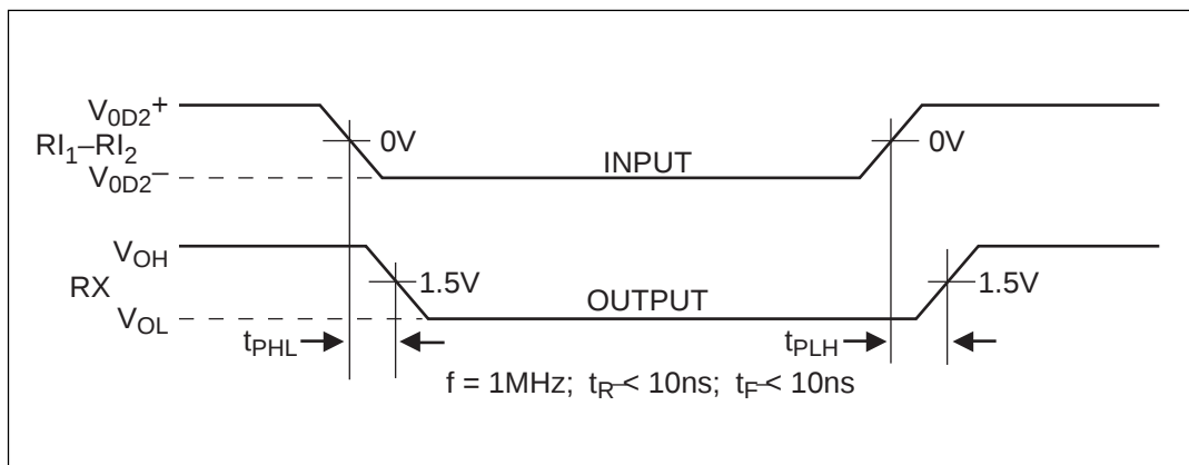
Figure 5. Receiver Propagation Delays
