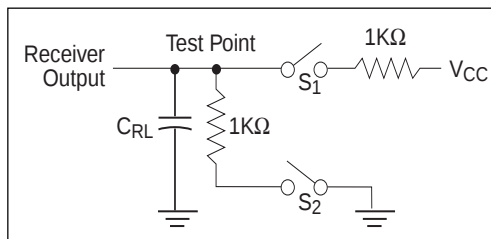
Figure 2. Receiver Timing Test Load Circuit
