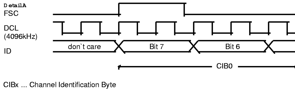
Figure 45 General Timing
