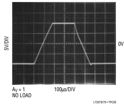
Large-Signal Transient Response V_S = \pm 15V
