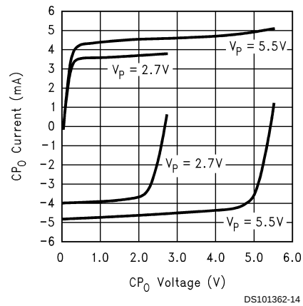
Charge Pump Current vs V_{CP0} Output
