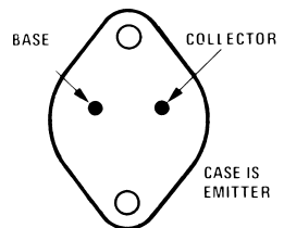
TO-3 Metal Can Package
