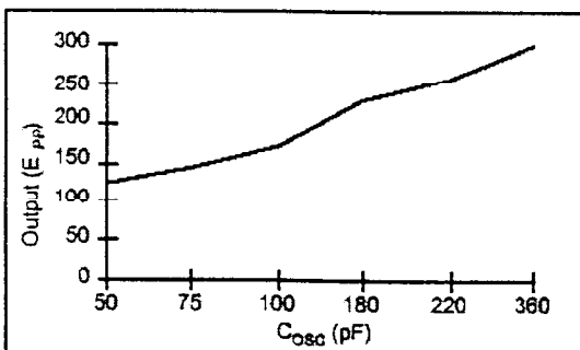
Output Voltage vs C_{osc}
