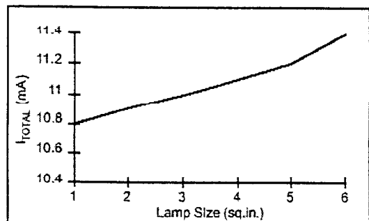
I_{TOTAL} vs Lamp Size
