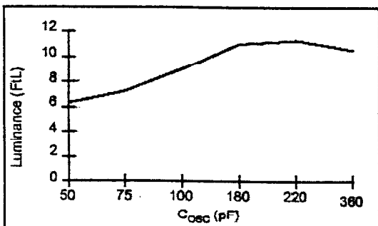
Luminance vs C_{osc}
