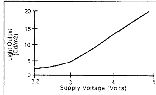
Luminance vs. V_{DD}=V_{coil} V_{DD}=3.0V ; Coil=5mH, 18 \Omega ; Load=10nF
