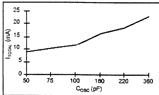
I_{TOTAL} vs C_{osc}
