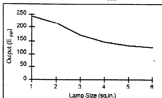
Output Voltage vs Lamp Size.
