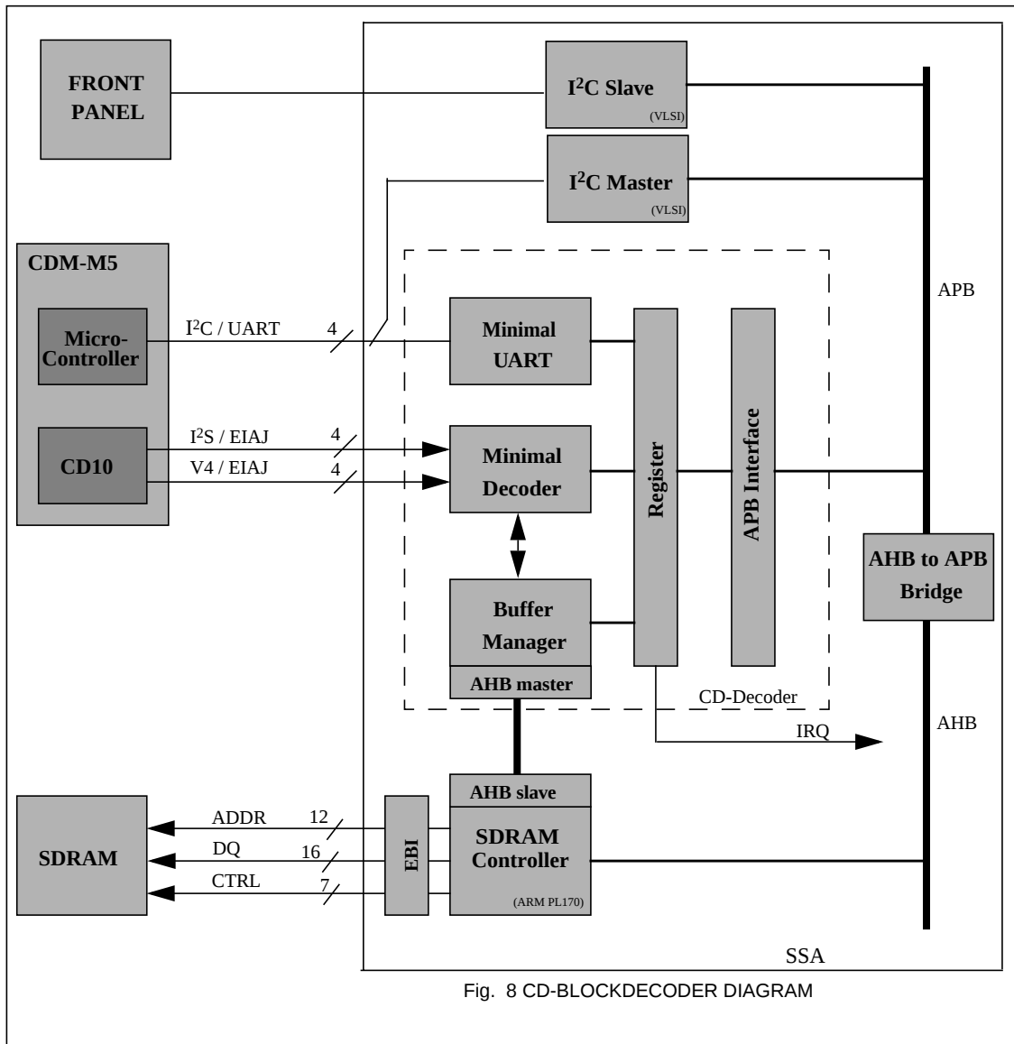
Block Diagram (1)
