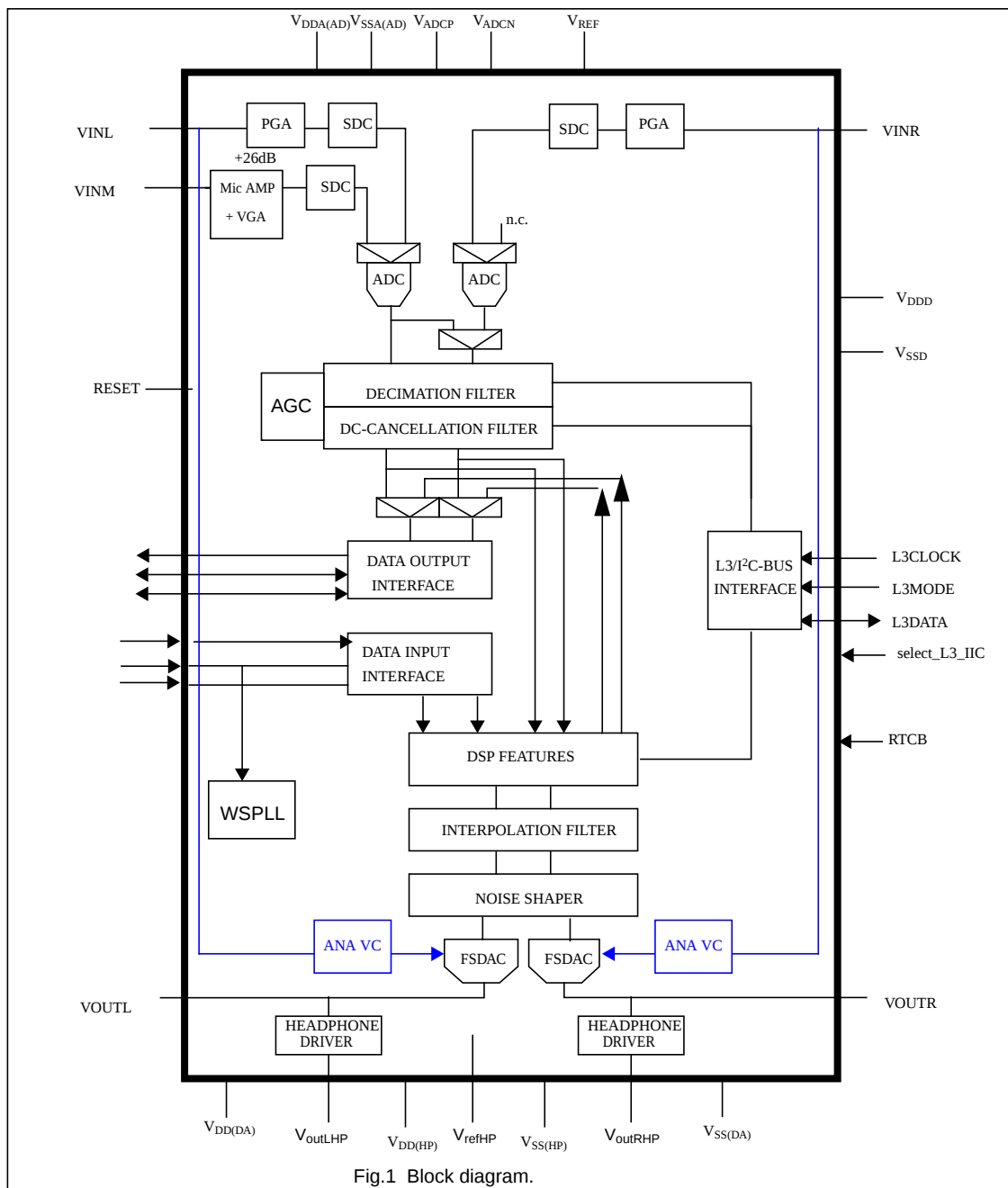
Fig.1 Block diagram.
