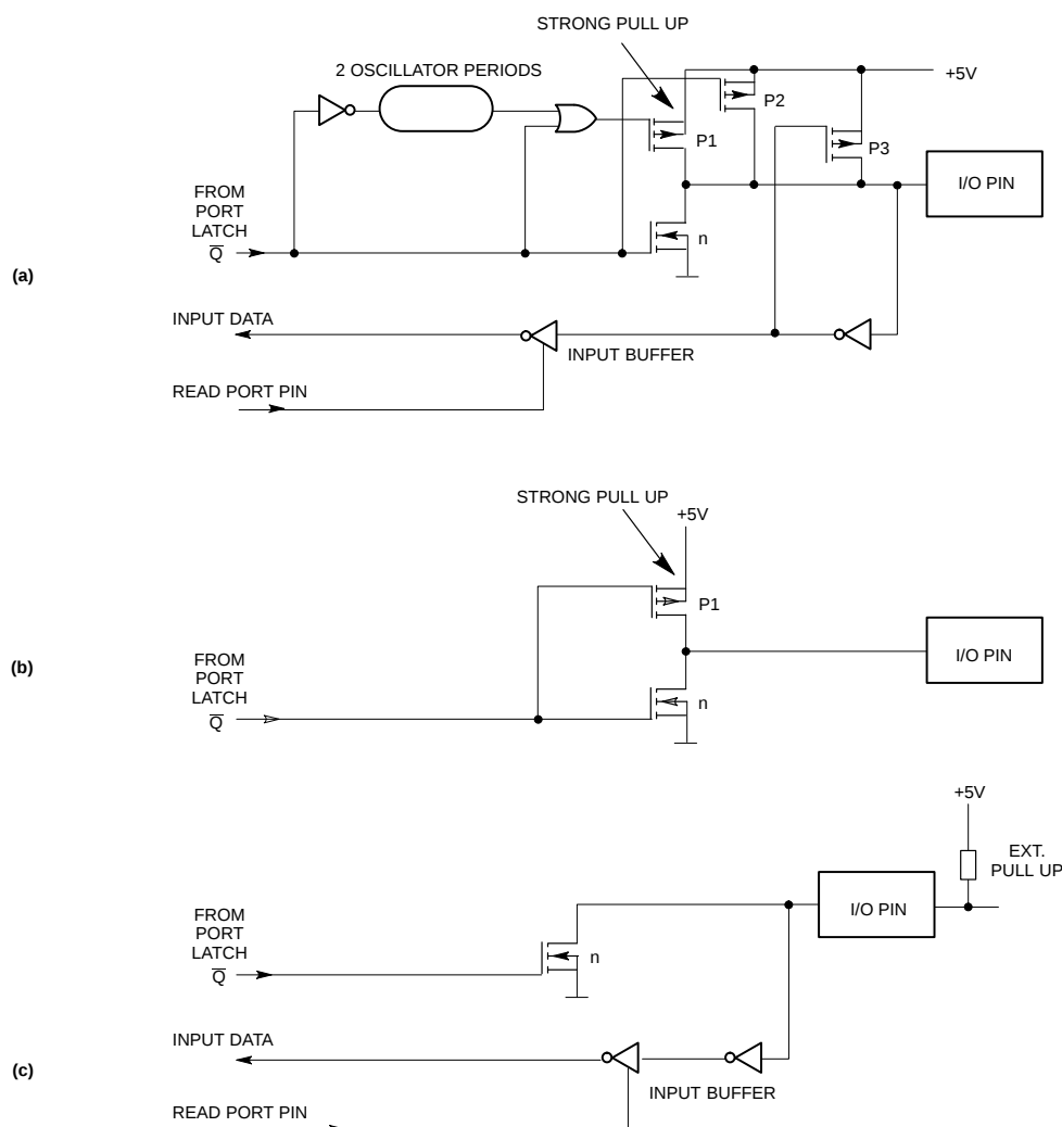
Figure 3. Ports
