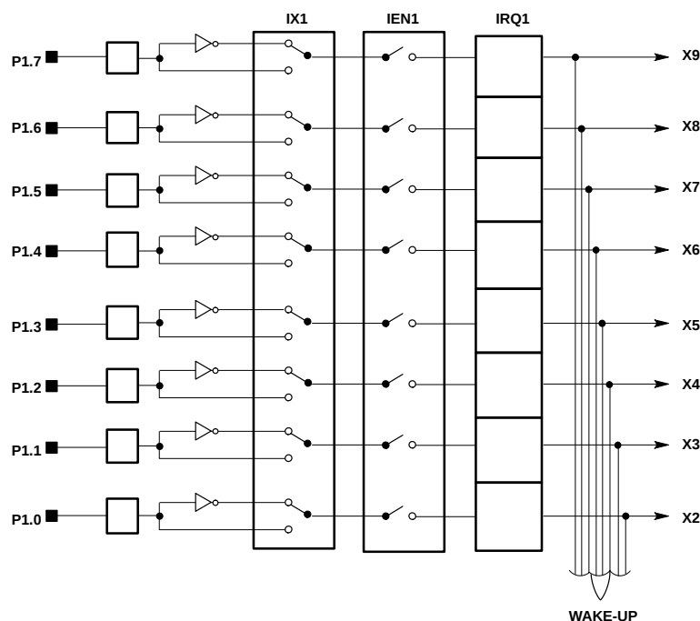
Figure 12. External Interrupt Configuration
