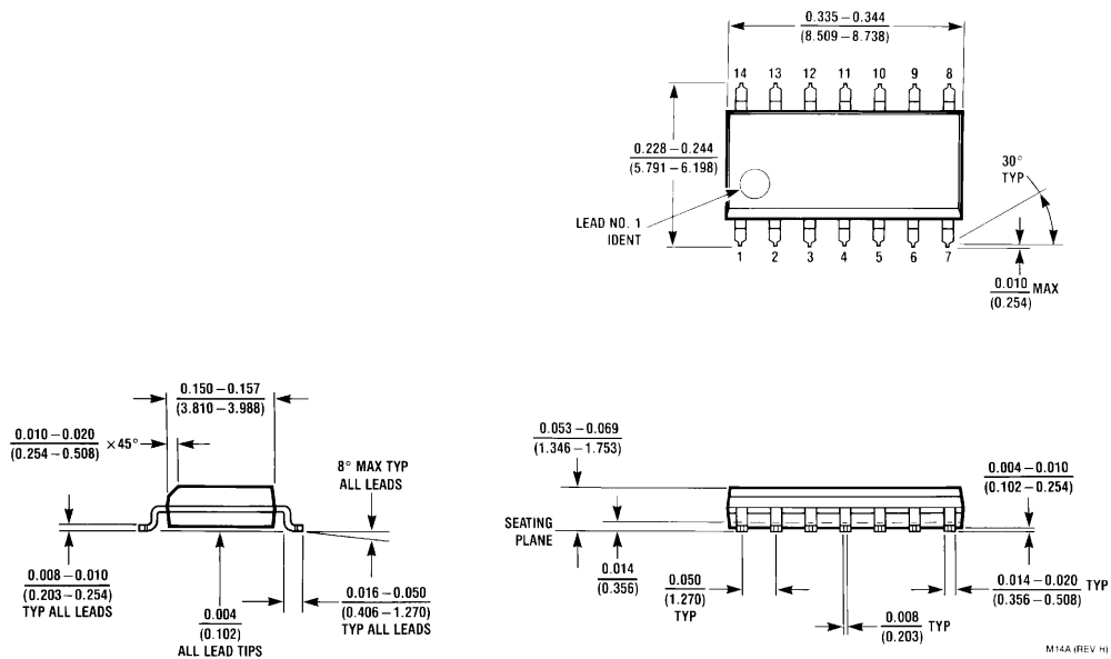
Molded Package (SO) Order Number LM837M NS Package Number M14A
