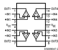
Dual-In-Line Package
