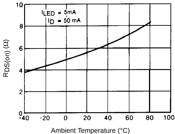
Figure 4. Typical On-Resistance
