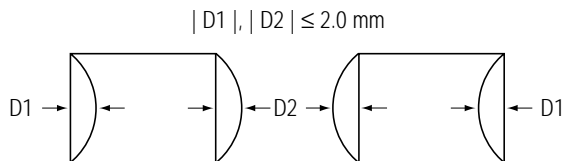
Figure 4-5. Pinbalance
